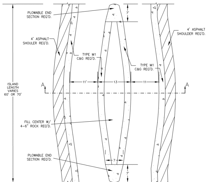
Figure 3: Detail Drawing of Center Island
